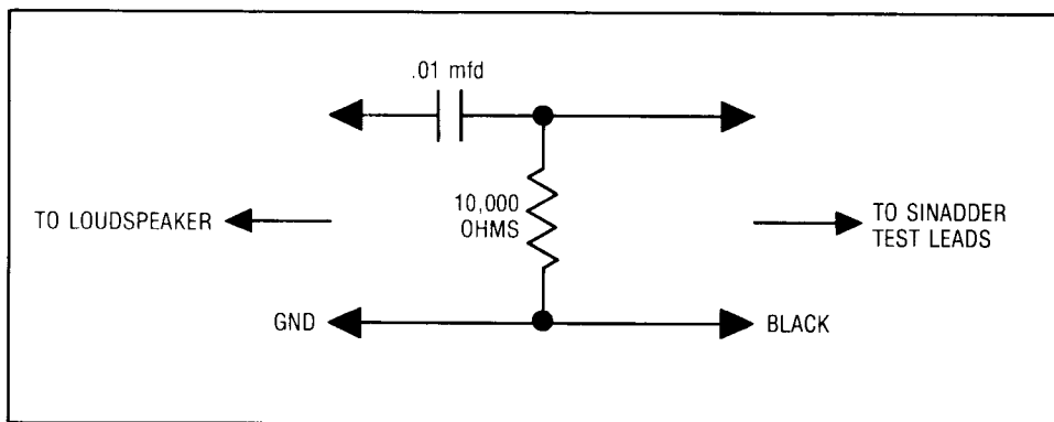
Auxiliary Filter Circuit
