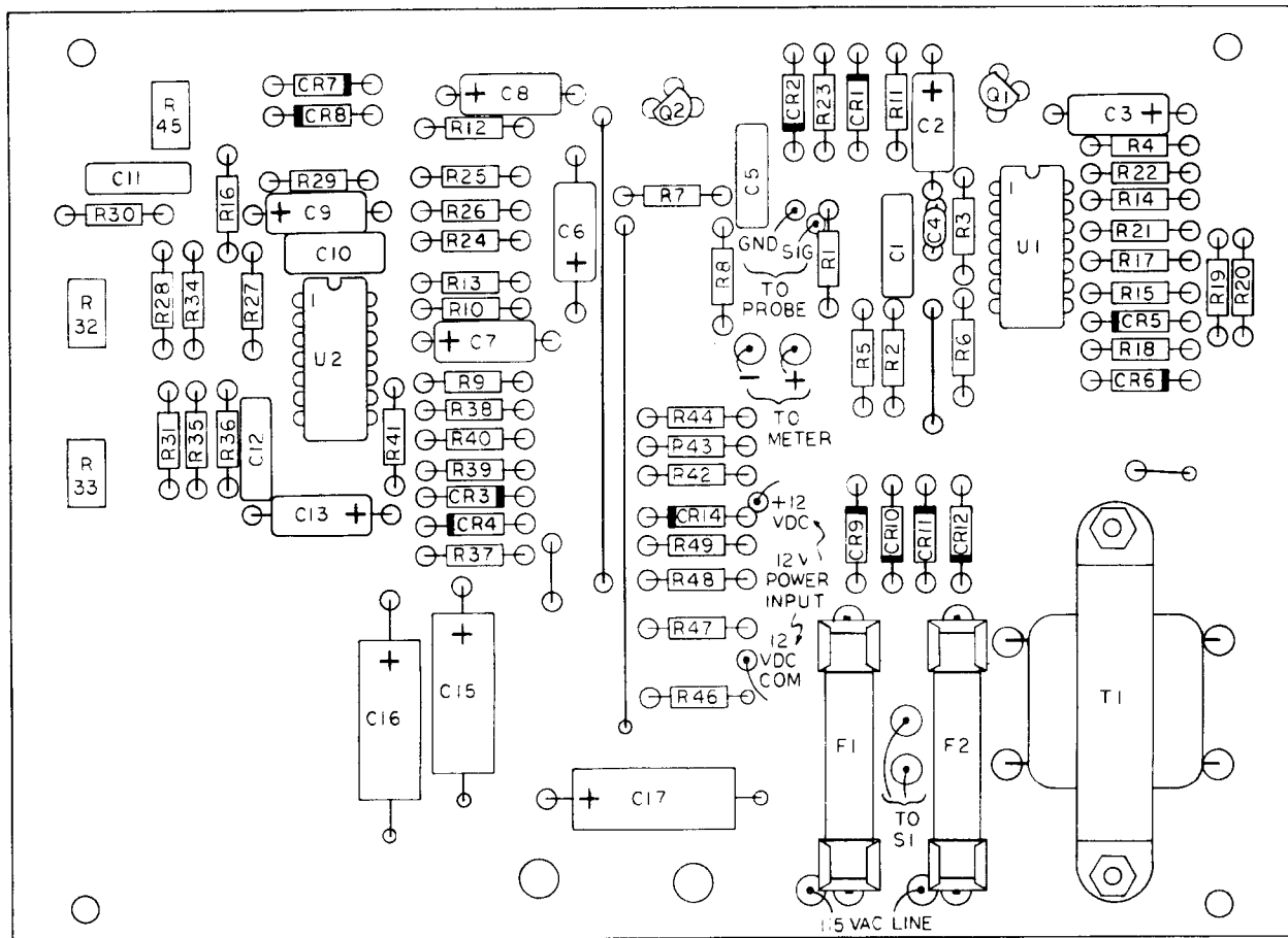
Figure 4. SINADDER™ Circuit Board with Components.
