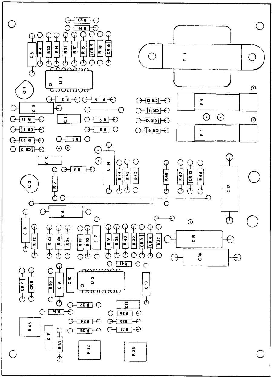
Figure 4. SINADDER™ Circuit Board with Components.
