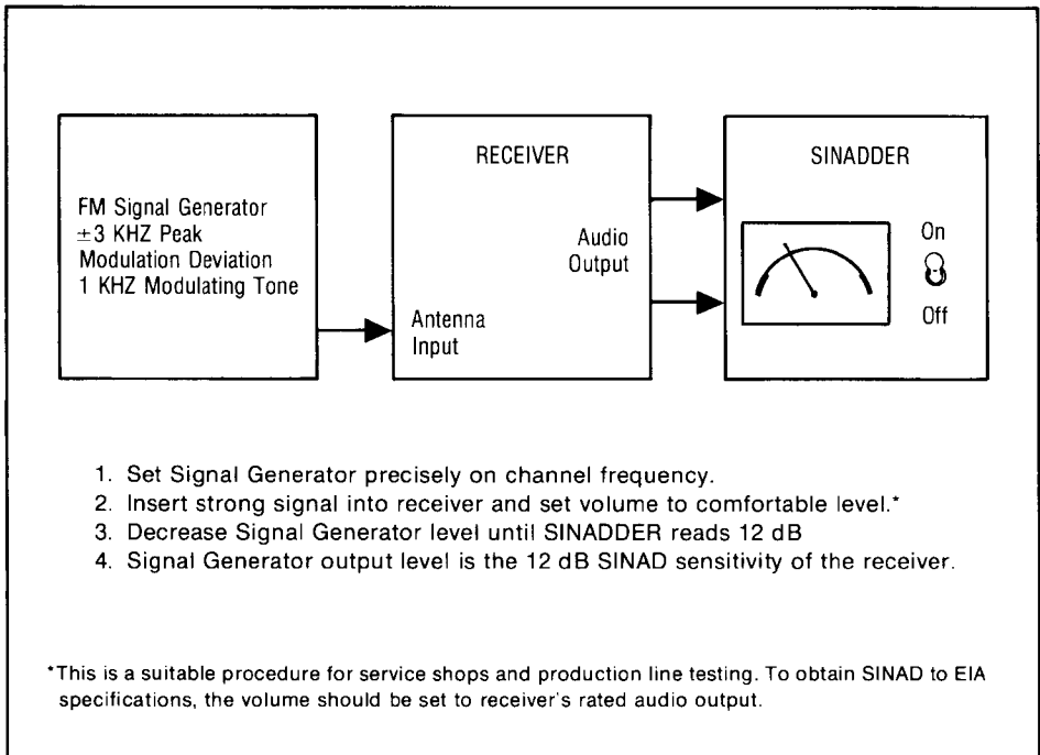
Figure 2. SINAD measurement using the SINADDER™
