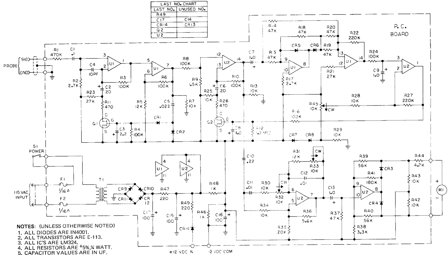
Figure 3. SINADDER™ Schematic Diagram
