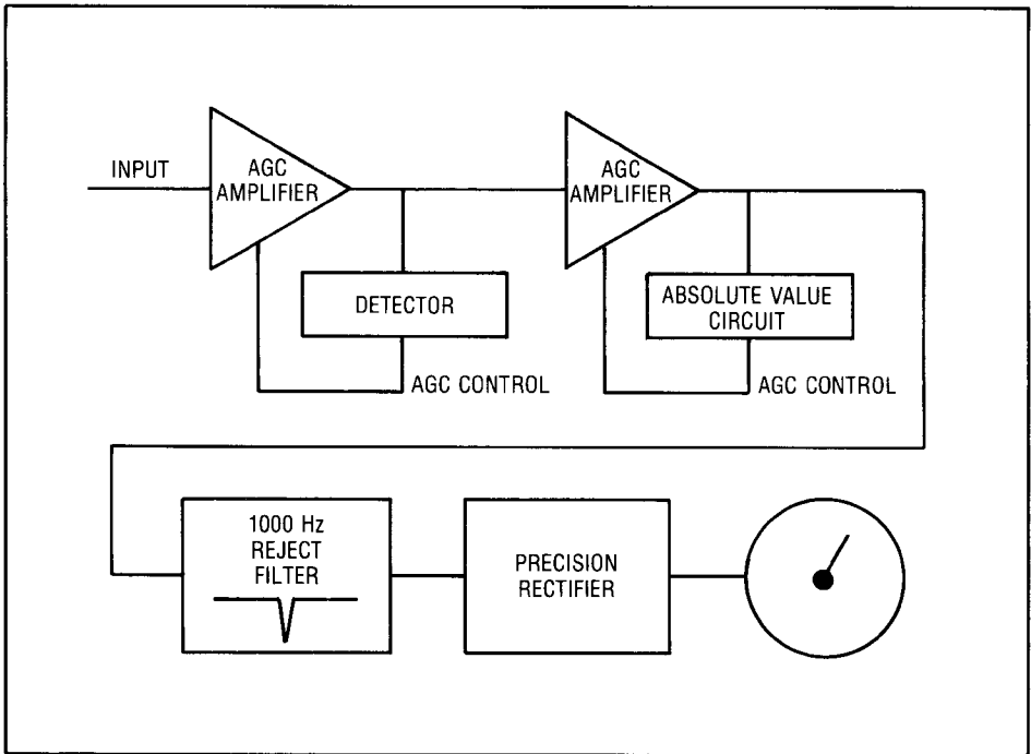
Figure 1. SINADDER™ Block Diagram
